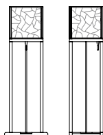
52612 Stand con lampada colore ambra lamp stand amber colour cm 45 x 35 X h 136 in 17 3/4 x 13 3/4 X h 53 1/2
