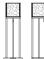
52611 Stand con lampada colore grigio lamp stand grey colour cm 45 x 35 X h 136 in 17 3/4 x 13 3/4 X h 53 1/2
